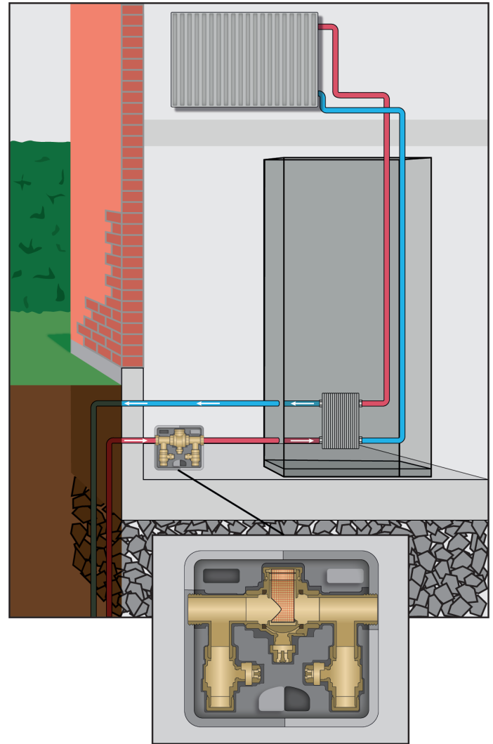
Filling device 752 1" - 1 1/4"
